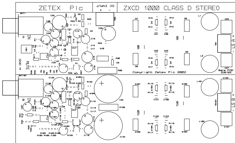
Fig.1. Component Overlay
