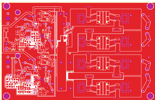
Fig.2. Top Copper
