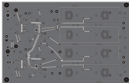
Fig.3. Bottom Copper
